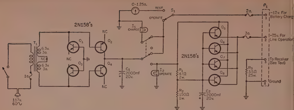
Fig. 1—Circuit of the transistorized battery charger and eliminator built into an LMB case #W-1A. All capacitors are in mf.
