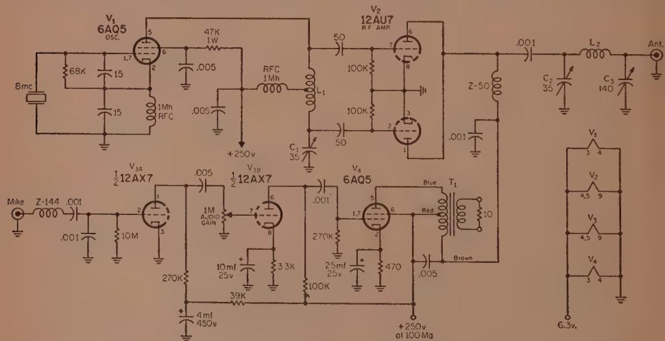
Fig. 1—Schematic diagram of the 10 watter for 6. The 12AU7s act as push-push doublers providing output 50 mc from 8 mc crystals and require no neutralization. The modulator is straight-forward and can be employed separately in other transmitters with no more than 10 watts in the final. Coil data may be found in the text.
