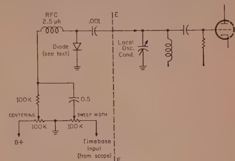
Fig. 3—Detailed circuit of the reactance modulator. Components to the right of line EF already exist in the receiver. Components to the left of line EF are added to form the reactance modulator.
