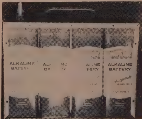
Typical installation of four Eveready 7.5 volt Alkaline batteries. In this unit, a two meter portable transceiver, provision is made to charge each battery through a separate dropping resistor. All batteries are connected in parallel in operation.
