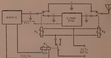
Fig. 1—Circuit of d.c. relay hookup when using KWM-1 with a linear amplifier. Relays K_1 and K_2 are conventional 110 v.a.c. coaxial relays. Relay K_3 is a 10,000 ohm d.c. relay requiring 10 ma or less for pull-in.
