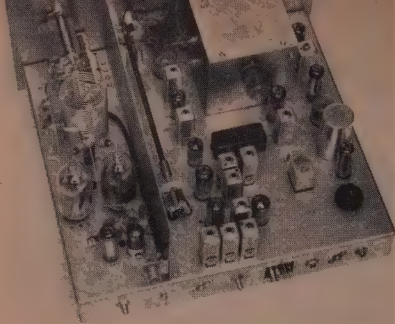
Top chassis view of the Galaxy 300. The dual v.f.o. is in the box at the upper right with the Compactron oscillator tube protruding from one side of it. The crystal filter is in the small black box just behind the v.f.o. The capacitor with the long shaft tunes the transmitter mixer. The final amplifier compartment is at the left. The two 6HF5 tubes are at the center with the 0A2 regulator and the 6BZ6 r.f. amplifier toward the chassis apron. The final bandswitch is inside of the lower part of the tank coil.
