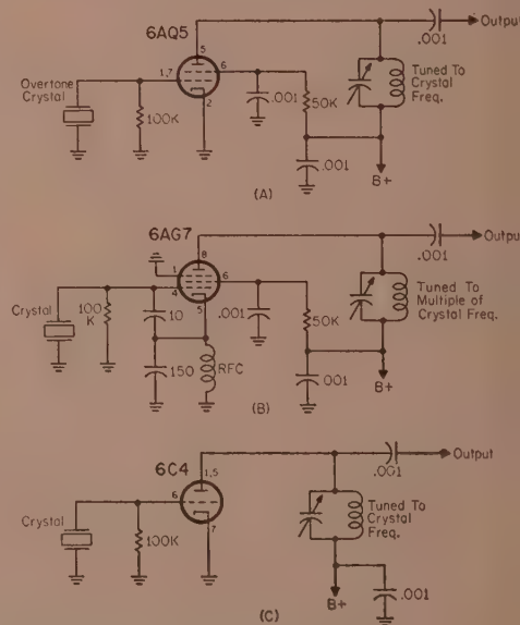
Fig. 1 (A) Conventional crystal oscillator using a tetrode giving output at the crystal frequency. (B) An oscillator used to obtain output at some multiple of the crystal frequency. (C) A circuit often used in receiving applications and in v.h.f. converters.
