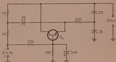
Fig. 2—Transistorized 1 kc oscillator. Q 1 may be a 2N1175, 2N632, 2N324 or 2N109.
