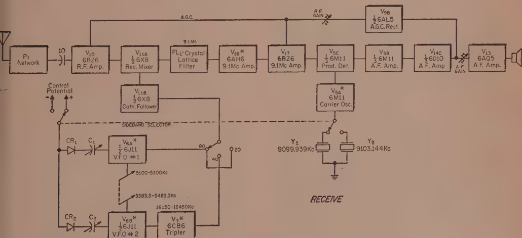
Fig. 2—Functional block diagram for the receiver section of the Galaxy 300 Transceiver. Elements common to both transmit and receive are marked (*). Receiver mixer ( V_{11A} ) input circuit is bandswitched with fix-tuned circuits.
