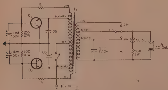
Fig. 1—Circuit recommended by Triad for a 115 v.a.c. power supply using their transformer type TY76A. Any of the listed transistors may be used with the proper value of R 1 as shown in the chart.
