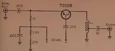
Fig. 2—Simple one transistor 6 meter preamplifier providing 12 db gain. Coil data may be found in the text. All capacitors are in mf unless otherwise stated and all resistors are ½ watt.
