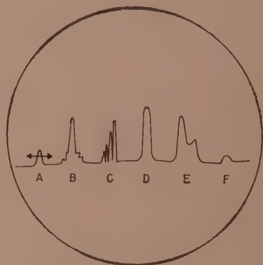
Fig. 1—Typical Panoramic display on the c.r.t. screen. Different types of signal are shown (A) represents "calibration pip" which is variable in position and used for frequency checking.
