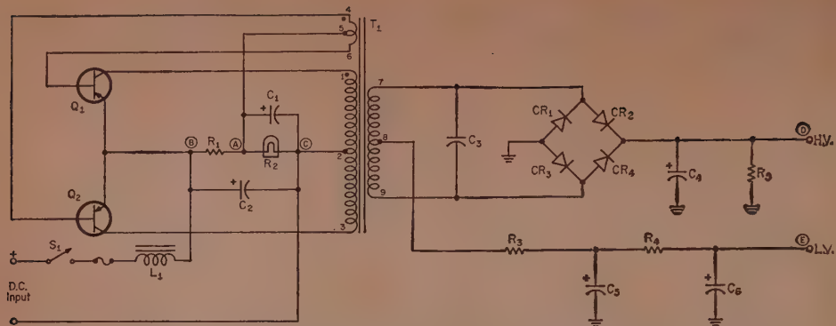
Fig. 1—Circuit of a d.c. to d.c. converter. When properly designed, it will start oscillating in a wide range of temperatures, from -50^{\circ}\text{C} to 70^{\circ}\text{C} and provide a high and low voltage output.
