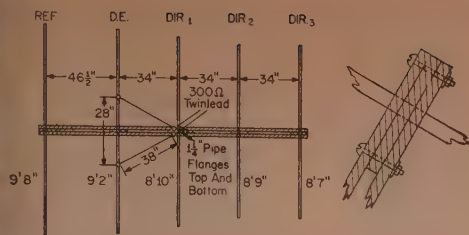
Fig. 1—A simple 5 element 6-meter beam used at W8ZCV. The beam is mounted to the mast by means of a pipe flange at the center of the boom. See text for details.
