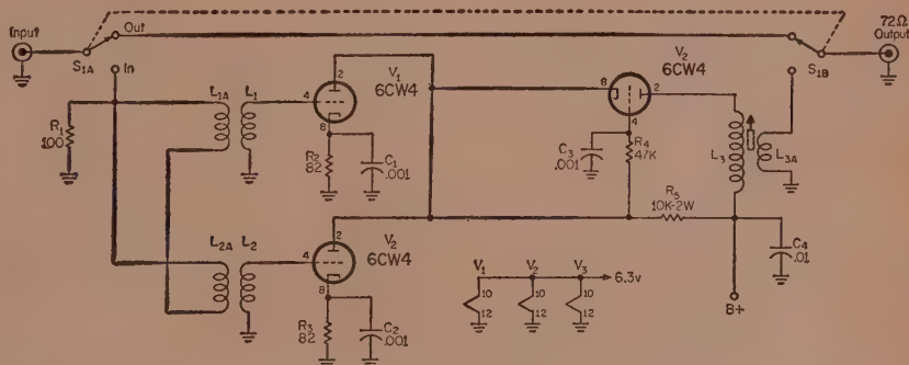
Fig. 2—Circuit of a 3 nuvistor broadband r.f. amplifier. All capacitors are in mf and are disc ceramics. All resistors are 1/2 watt unless otherwise noted.
