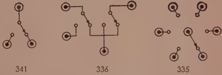
Fig. 1—Schematics of the Waters coax switches.
