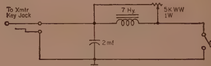
Fig. 1—Key click filter for the Heath HX-10 Marauder Transmitter.
