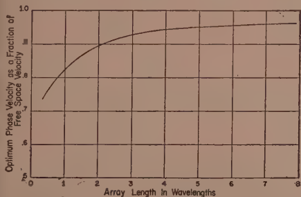
Fig. 2—Chart showing how the optimum phase velocity increases with length for a yagi. Free space velocity (velocity of light) is indicated by the dotted line.
