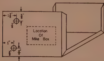
Fig. 1—Diagram showing lower portion of cabinet. Drill as indicated. Location of the carbon mike "box" is not critical, hence exact dimensions are not shown.
