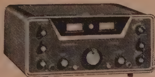
SR-150 TRANSCEIVER
