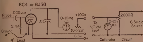
Fig. 2—A simple v.t.v.m. that may be used to measure the signal voltages at the #1 and #3 grids. Also shown is a simple set-up that may be used for calibration
