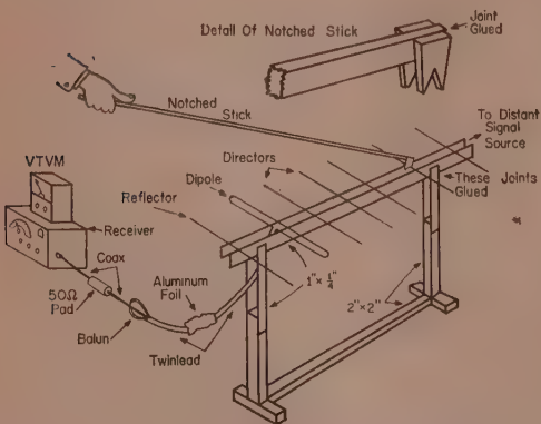
Fig. 4—Suggested experimental setup for developing optimum yagis.
