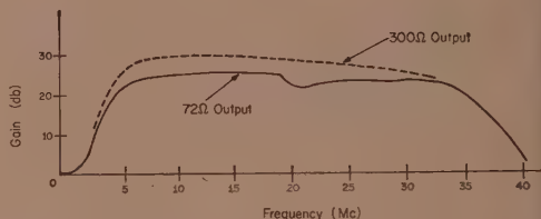
Fig. 1—Plot of gain vs frequency. Coil L_2 covers up to 22 mc and L_1 covers from 15 to 40 mc. To peak the center, L_3 is tuned to 20 mc to cover from 15 to about 23 mc.
