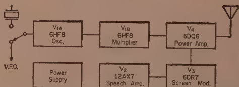
Fig. 1—Block diagram of the Knight-Kit T-60 Transmitter, available from Allied Radio for $49.95.
