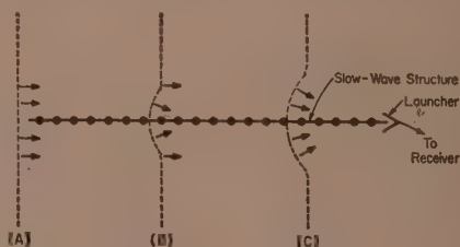
Fig. 1—Action of the incoming wavefront as it encounters the slow-wave structure. As the plane wavefront moves toward the launcher, a dent is gradually produced, (B) and (C), causing the r.f. energy to converge onto the feed as indicated by the arrows.
