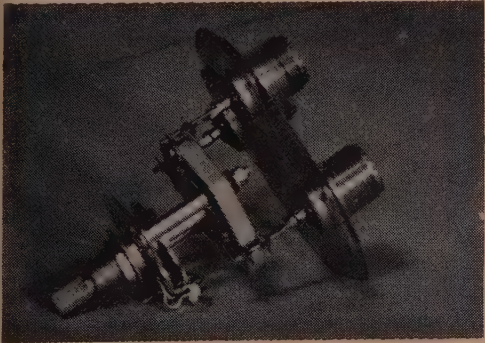
The switches are sealed in steel cans and to even see the switch mechanism, a can opener must be resorted to. Note the double wiper contact on the ceramic switch section.
