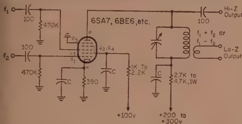
Fig. 1—An operational pentagrid mixer circuit is shown above. Bypass capacitors C can be 0.005 mf if all frequencies involved are higher than 400 kc. If the output frequency is within 25% of f_1 or f_2 , a double tuned output circuit is recommended. All resistors are \frac{1}{2} watt unless otherwise noted and all capacitors are in mmf.
