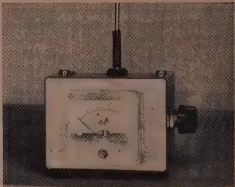
The Delphi Model 112 field intensity meter.
