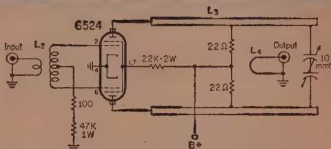
Schematic diagram of K9DTB's 432 mc tripler. Unit can be constructed in a 3 x 4 x 10" chassis.
