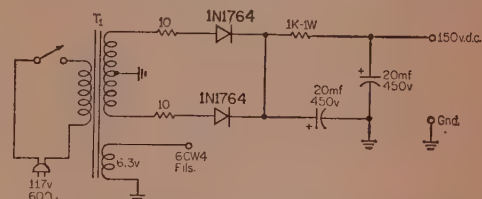
Fig. 3—This simple power supply may be used if power is not available from the accessory socket. Transformer T_1 is a Stancer PS8416 or equal.
