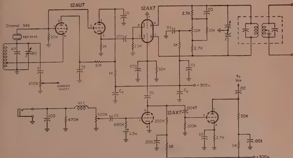
Fig. 1—Revised circuit of the W3JHR s.s.b. generator.
