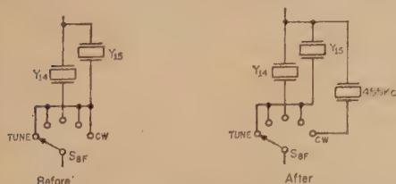
Fig. 2—Circuit modifications necessary for the insertion of a 455 kc crystal for improved c.w. operation.
