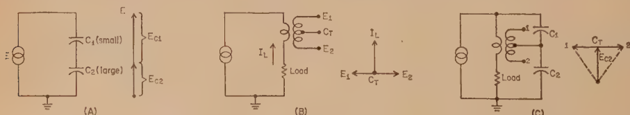
Fig. 2—(A) Capacitive voltage divider and its phase relationships; (B) Current sensing with a transformer; (C) Combination; with the net voltage outputs shown by dotted lines.
