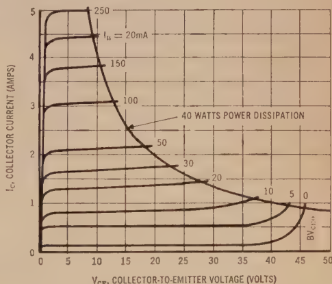
Fig. 1—Typical power transistor output characteristics, Motorola 2N1530.
