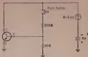
Fig. 3—Simple transistor beta checker. Comparison is made between collector current with and without switch S closed. Battery polarity shown is for p.n.p. transistors and should be reversed for n.p.n. types.
