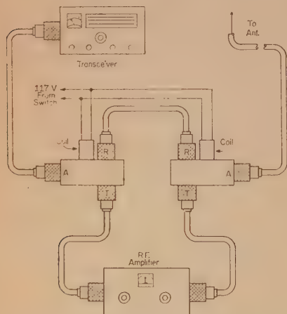
Fig. 3—Relays K_3 and K_4 of the antenna switching unit in fig. 2 may be replaced with coaxial-type relays shown here. In this case, S_1 will require an extra set of contacts for the a.c. power.
