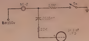
Fig. 3—A simple relaxation type oscillator developed by DL4VG (W9YUE). Care must be taken to keep the leads short.
