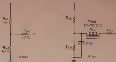
Fig. 7—Circuit of the low-pass filter to reduce harmonic content of the tone oscillator.
