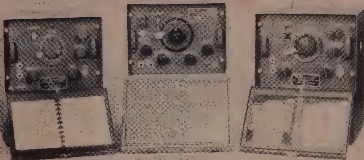
Shown here are three different versions of the BC-221. From l to r, BC-221M made by Bendix, the BC-221AN made by Cardwell, the very latest model and the BC-221F made by Zenith.
