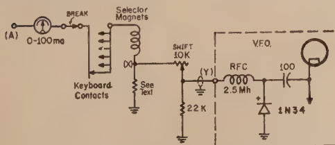
Fig. 1—Frequency Shift Circuit for the AN/ART-13.
