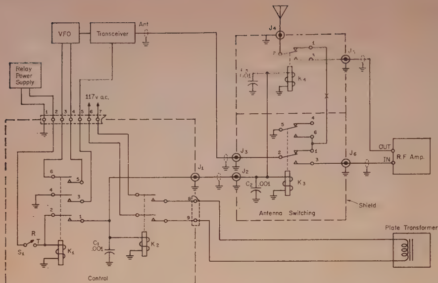
Fig. 2—Diagram of an antenna switching unit designed for the v.h.f. man, capable of one-switch operation of a transceiver with an auxiliary r.f. amplifier. Switch S_1 may be remotely located. Operation of v.f.o. and the transceiver itself are also included. All capacitors are .001 mmf disc ceramics. See text for relay information. An r.f. preamp for the receiver can be inserted at point X if desired.
