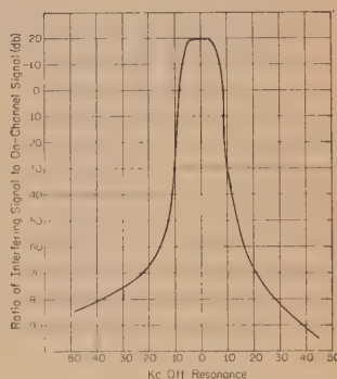
Fig. 3—Two-signal selectivity of a typical h.f. communications receiver.
