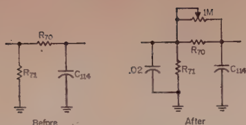
Fig. 8—Circuit modifications necessary to permit adjustment of the keying time constant.
