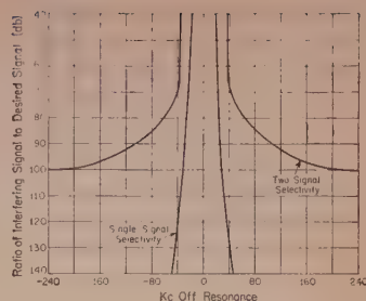
Fig. 1—Comparison of single-signal and two-signal selectivity of a typical v.h.f. receiver.
