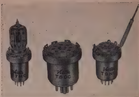
Vector adapters for measuring voltage and resistance from the top of a chassis. The socket and plug sections are connected together directly with test point terminals brought out from each pin.
