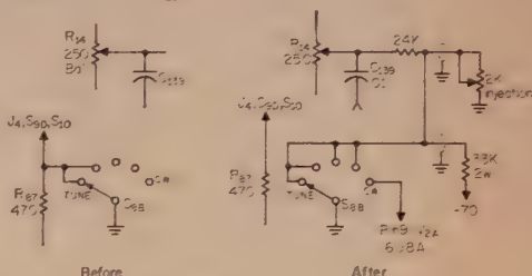
Fig. 3—Circuit modifications for the Injection control, ganged to the Mic. Gain pot. The Mic Gain circuit is unchanged and is not shown.
