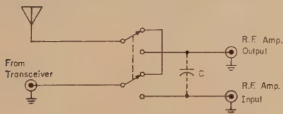
Fig. 1—Diagram illustrating a simple method of using an r.f. power amplifier in conjunction with a transceiver. "C" is the stray capacity develops across the switch. (See text).
