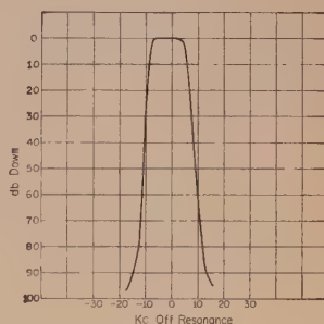
Fig. 2—Single-signal selectivity of a typical h.f. communications receiver.
