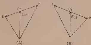
Fig. 4—(A) The unbalance in output voltages (dotted lines) with the leading (capacitive) current in the transmitter load; (B) Same, with lagging (inductive) current.
