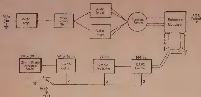
Fig. 1—Block diagram of the W2WZR direct sideband phasing rig for the two meter band.
