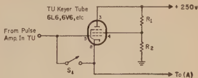
Fig. 2—Typical Keyer Tube Circuit in a TU.
