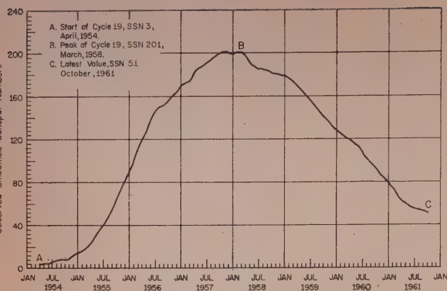
Fig. 1—Graph illustrating the progress of Sunspot Cycle 19 from April 1954 to Oct. 1961.
