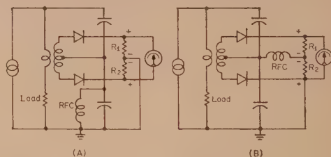
Fig. 3—(A) Practical coax phase detector showing added parts necessary for rectification and the output polarity developed across the load resistors; (B) Circuit re-arranged (Jan. 1962 CQ ) giving an output having one leg at d.c. ground potential.
