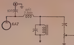
Fig. 1—Modification made in the plate of the mixer tube that will enable the additive-subtract system of frequency measurement to be used. This can provide a great increase in frequency meter accuracy. The mixer tube type will vary from model to model and may be a 6A7, 6K8 or a 7B8.
