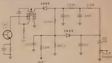
Fig. 4—Series type noise limiter for use in transistor receivers.
