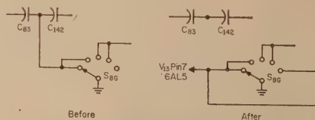
Fig. 10—Circuit modifications necessary to eliminate a.l.c. action in the c.w. mode.
