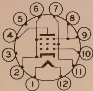
Fig. 1—Basing diagram of the 7984, a Compactron equivalent of the 6146. It is housed in a T-12 glass envelope and is of single end construction. It can deliver 46 watts output at 175 megacycles.
