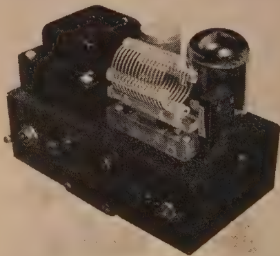
Top view of the one tube "Compactron" transmitter showing parts layout. The On-Off switch and key jack are to the left of the meter and the Plate and Antenna tuning controls are to the right.
