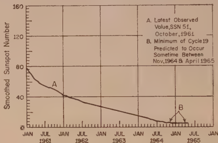
Fig. 2—Predicted smoothed sunspot numbers for the remainder of Sunspot Cycle 19 from October 1961 to May 1965. The actual sunspot minimum is expected to occur at B.
