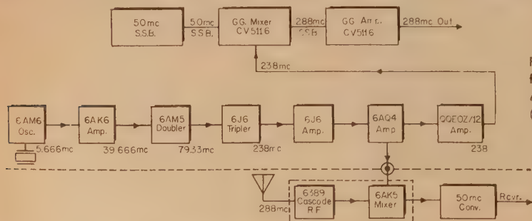
Fig. 2—Block diagram for the VK3EHL 288 mc sideband station. (Courtesy of Amateur Radio, Aust.)
