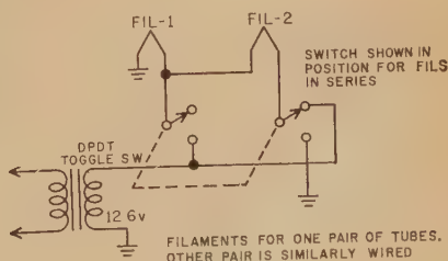
Fig. 2—Switching arrangement used to select circuit for 6 or 12 volt filaments.
