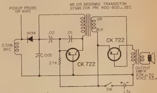
Fig. 1—Circuit of a simple keying monitor.
