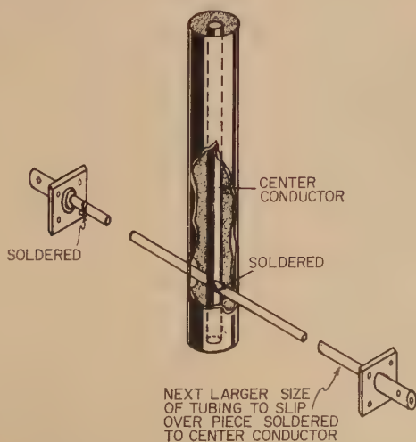
Fig. 2B—Wavemeter with input and output connection made to the center conductor.
