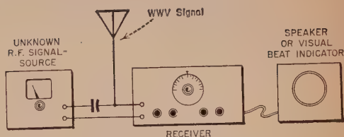
CALIBRATION OF L.F. SIGNAL SOURCE Fig. 1.
