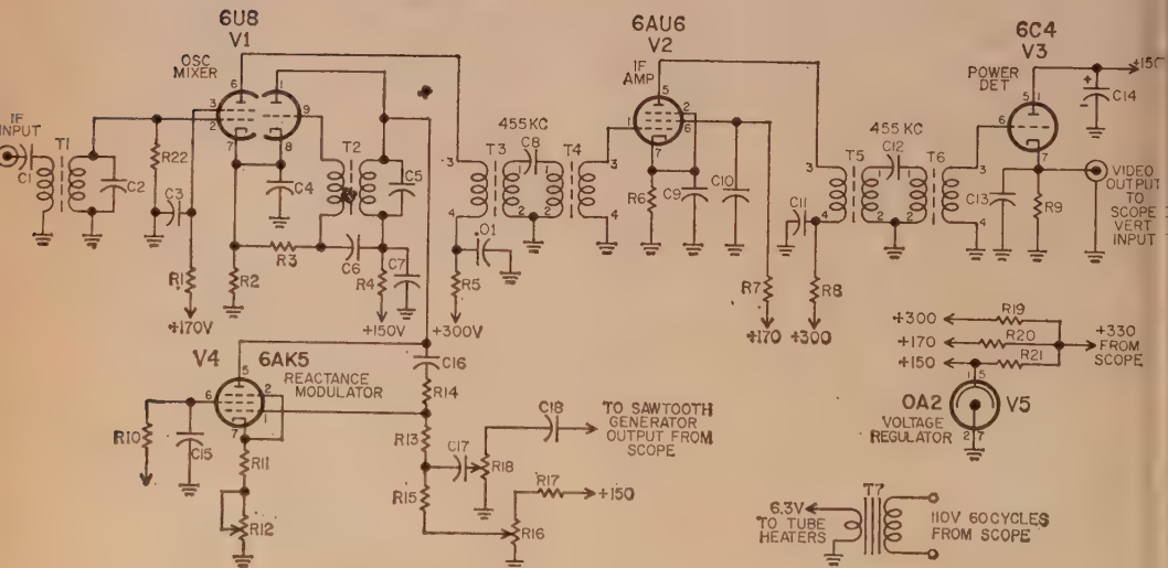
Fig. 1—Schematic diagram of the Pan-Scope.
