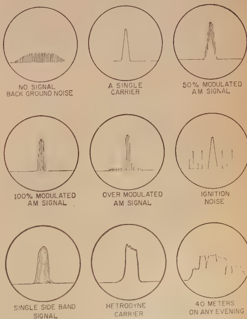
Fig. 5—Some typical Pan-Scope patterns.
