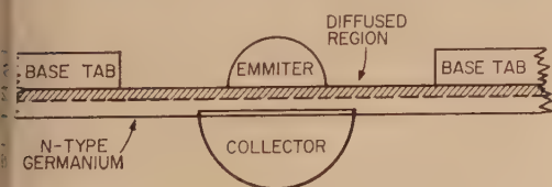
Fig. 1—Cross sectional view of the drift transistor structure.
