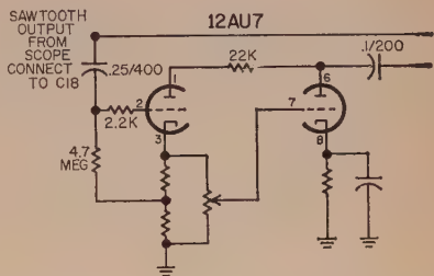
Fig. 3—Portion of the Heathkit O-12 oscilloscope showing the take off point for the sawtooth.
