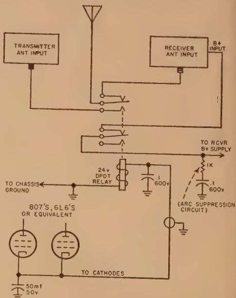
Fig.1 .—Simplified circuit of the cathode operated relay.
