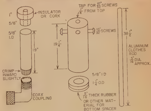
Fig. 1—Construction details and photos of the finished antenna for two meters.
