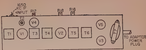
Fig. 2—Parts location; top view.
