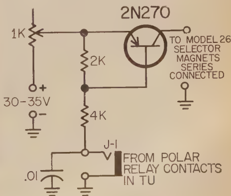
Fig. 1—W2JAV Transistorized Electronic Keyer for Model 26 Selector Magnets.
