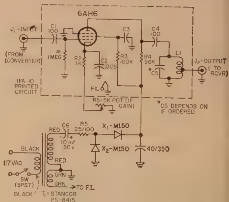
Fig. 1—A complete if amplifier for insertion between the converter and receiver. All parts shown within the dotted lines are part of a printed circuit kit marketed by International Crystal Co., 18 N. Lee, Oklahoma City, Okla. Desired operating frequency must be specified since it determines the value of L1 and C5.
