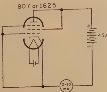
Fig. 1—Simple circuit used to test effectiveness of cathode and beam plate separation.
