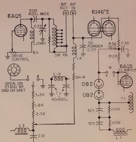
Fig. 4—Areas of the Viking II that were modified to accommodate the SB-10.
