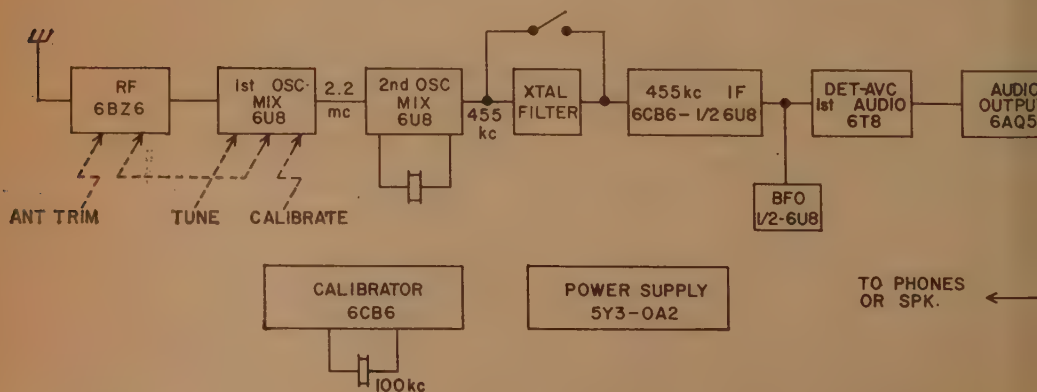
Fig. 1—Block diagram of the RME Model 4350A receiver.
