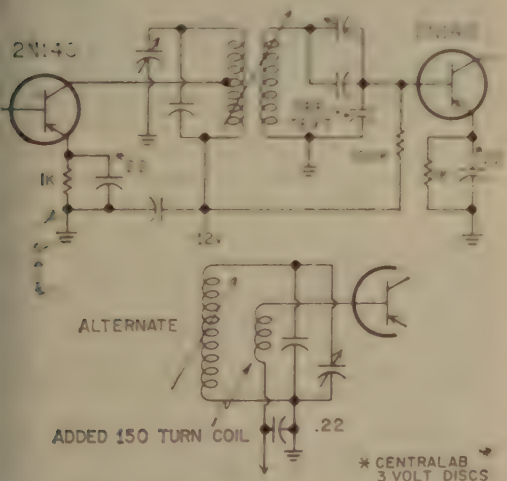
Fig. 1—Modifications of the BC-453 i-f transformers for use with transistors.
