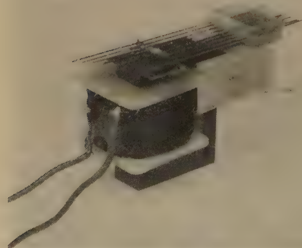
The Dixon Electronics resonant reed relay described in the text. There should be many applications for this device in Amateur radio. How about complete control of a transmitter from a remote location? You could control four servos with the eight channels available!
