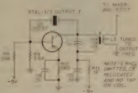
Fig. 2—Crystal controlled oscillator for the Mobile Converterettes (CQ, May 58)
