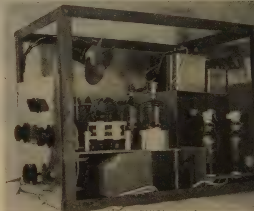
High-power amplifier in its chassis holding framework. Transformer at bottom lying on its side is a multi-filament type.
