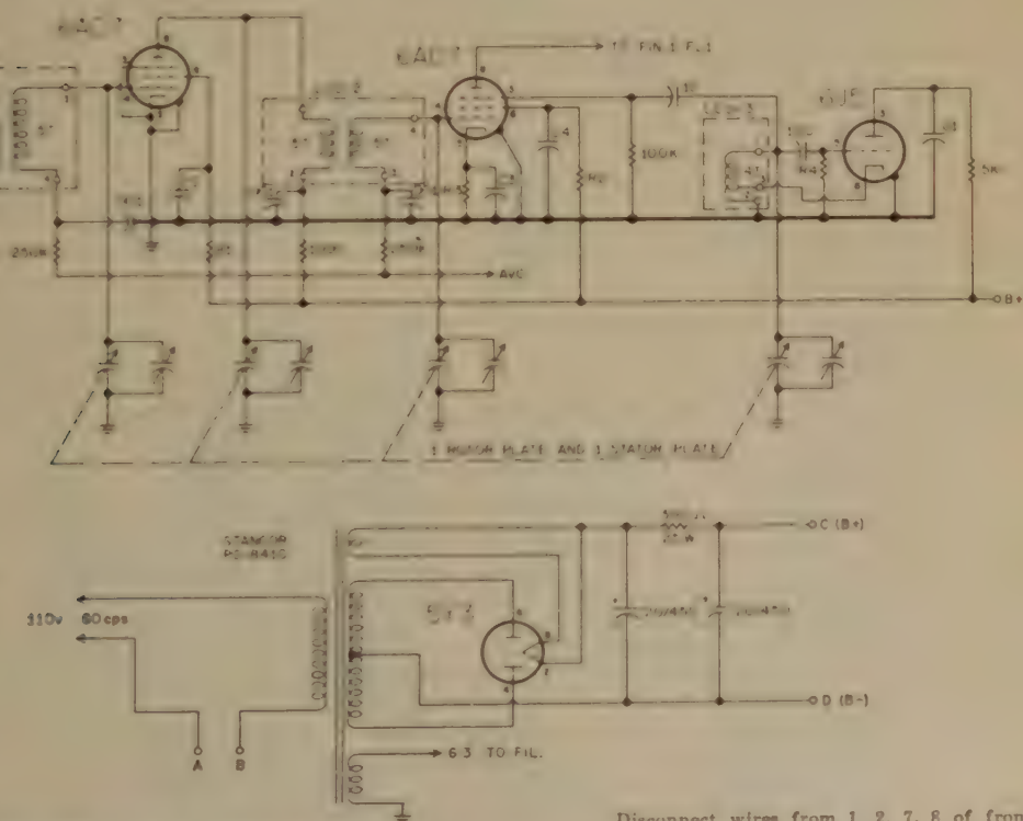
Fig. 2 Modified RF stages of BC-603 to 6 meters and power supply.
