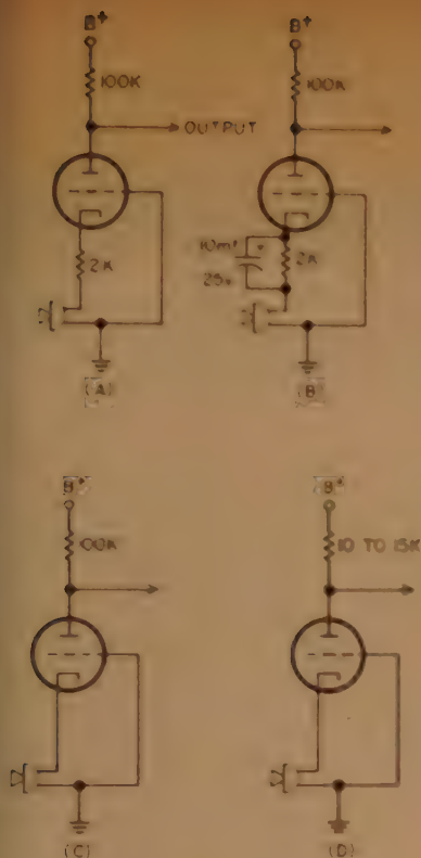
Fig. 1—Basic circuits for carbon microphone grounded grid preamplifiers as discussed in the text. (A) is the most common and yet the least efficient of the designs shown. The final version as concluded in the text is shown at (D). Tube is assumed to be half a 12AU7.
