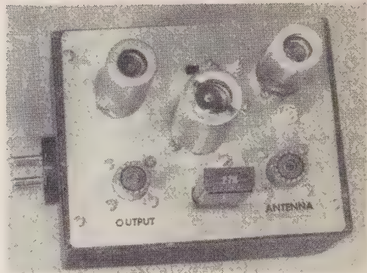
Fig. 1. Top view of the 21-Mc Converter showing the parts placement.
