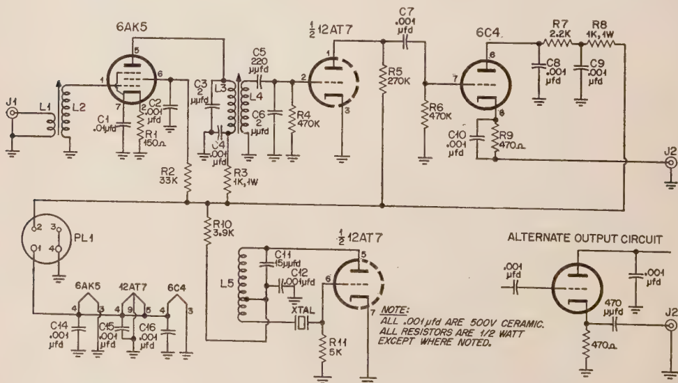
Fig. 2. Two outputs are shown, one for use where you have a d-c return through the antenna coil of the station receiver, and one for use where you are feeding a receiver input with no d-c return. Use the "Alternate Output Circuit" in the latter case.
