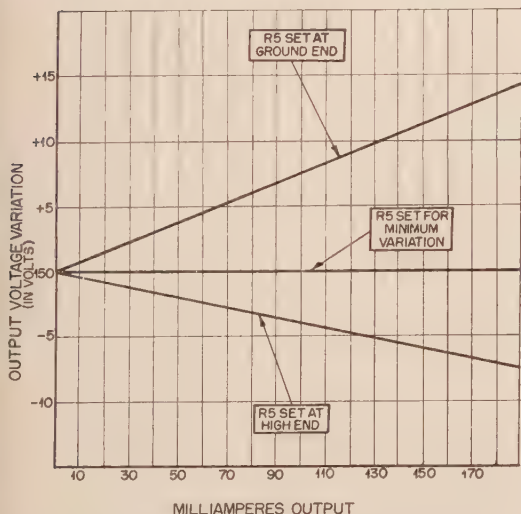
Fig. 3. The adjustment of R5 is important to the regulation, as can be seen from this graph. When R5 is properly set the variation in output voltage is difficult to detect, even over a wide current range.
