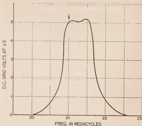
Fig. 4. Overall response curve of the converter when it is correctly adjusted.
