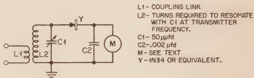
Fig. 1. Circuit diagram of a simple field strength meter, a most important piece of test equipment for adjusting linear amplifiers.
