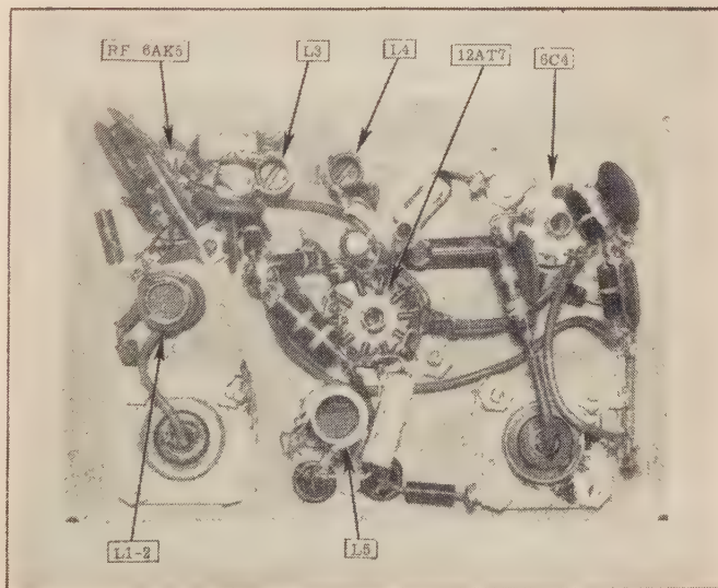
Fig. 3. Note short leads on parts. This results from careful placement of the mounted components.
