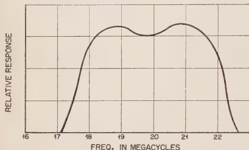
Fig. 5. Overcoupling can do this to the response.
