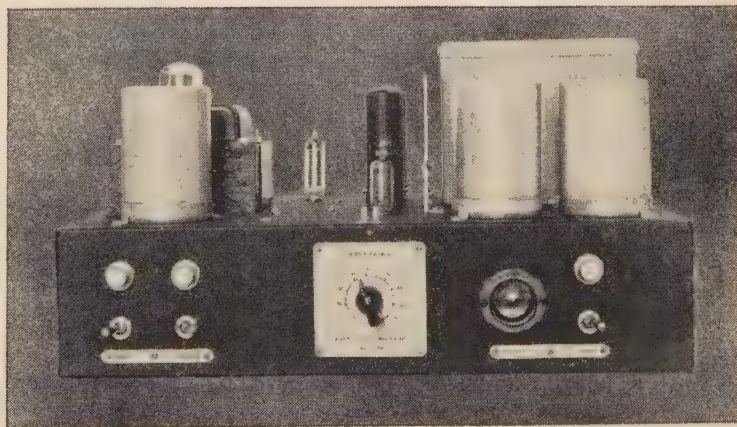
Front view of the power supply showing the loss-of-regulation "eye" indicator.
