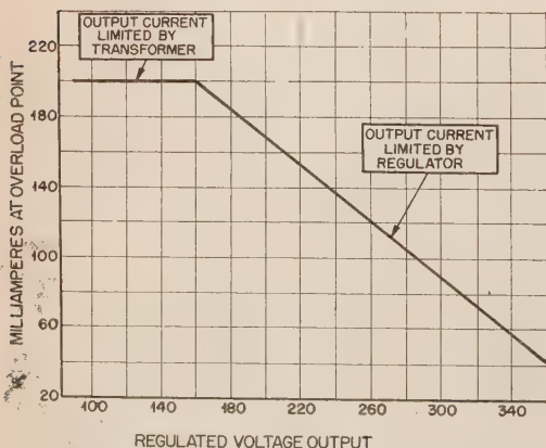
Fig. 2. Performance of the supply, showing the current capacity available at any specific voltage.
