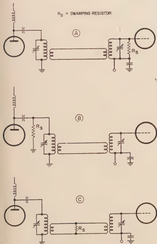
Fig. 2A-B-C. The swamping resistor (a non-inductive resistor) serves to reduce the power input to the amplifier and also stabilizes touchy amplifiers. Here are three points in the transmitter where it can be used.
