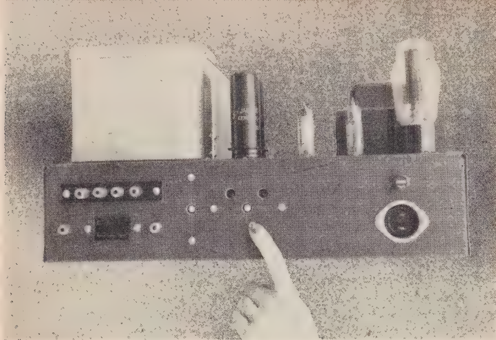
Rear of the regulated supply, R5 being pointed out.
