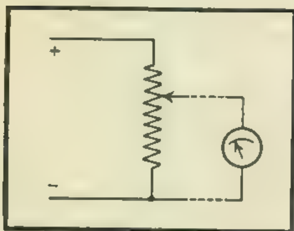
Fig. 1. Basic circuit for direction indicator potentiometer.
