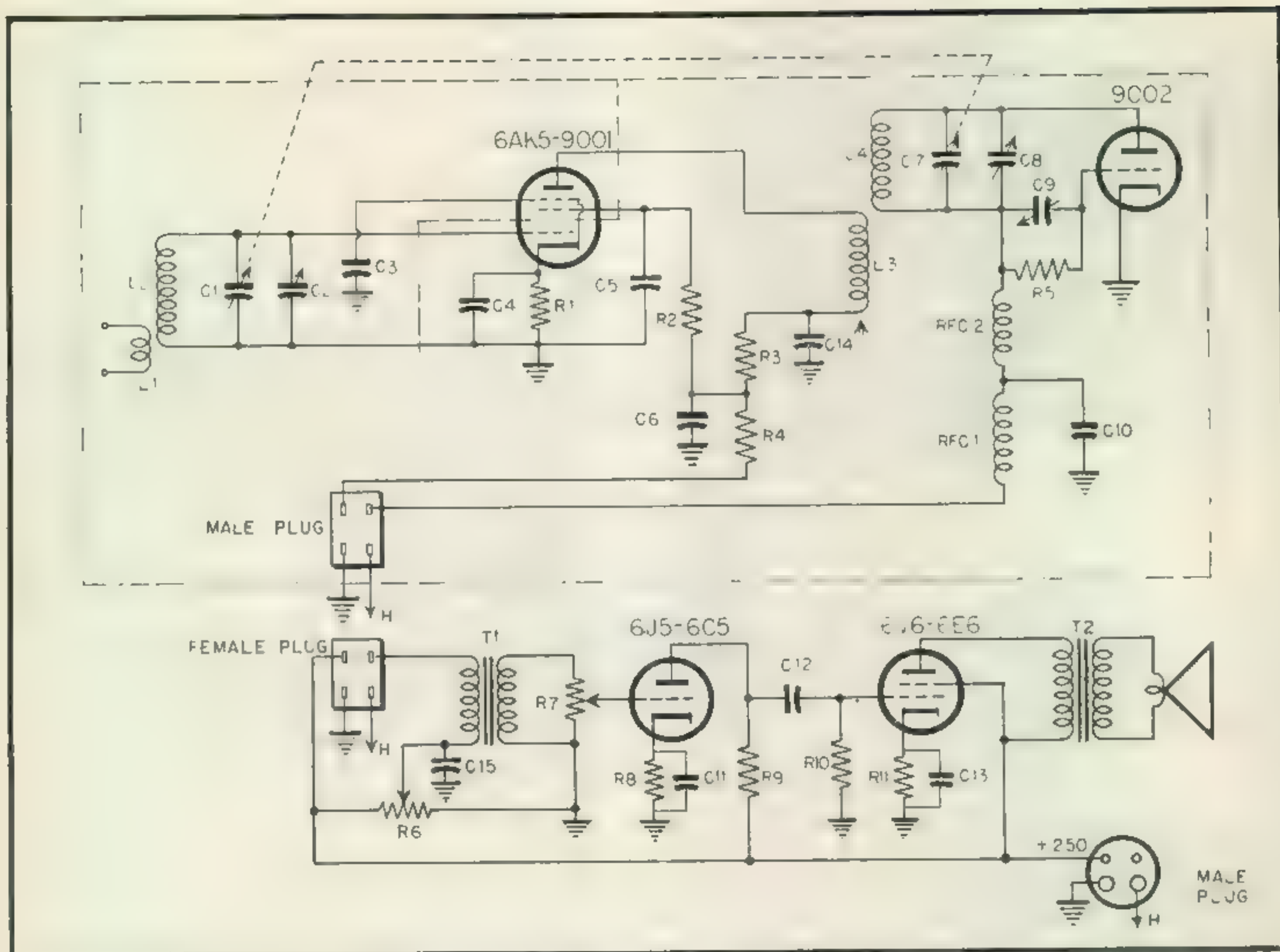
Circuit diagram of two-meter mobile receiver. Following is parts list.
