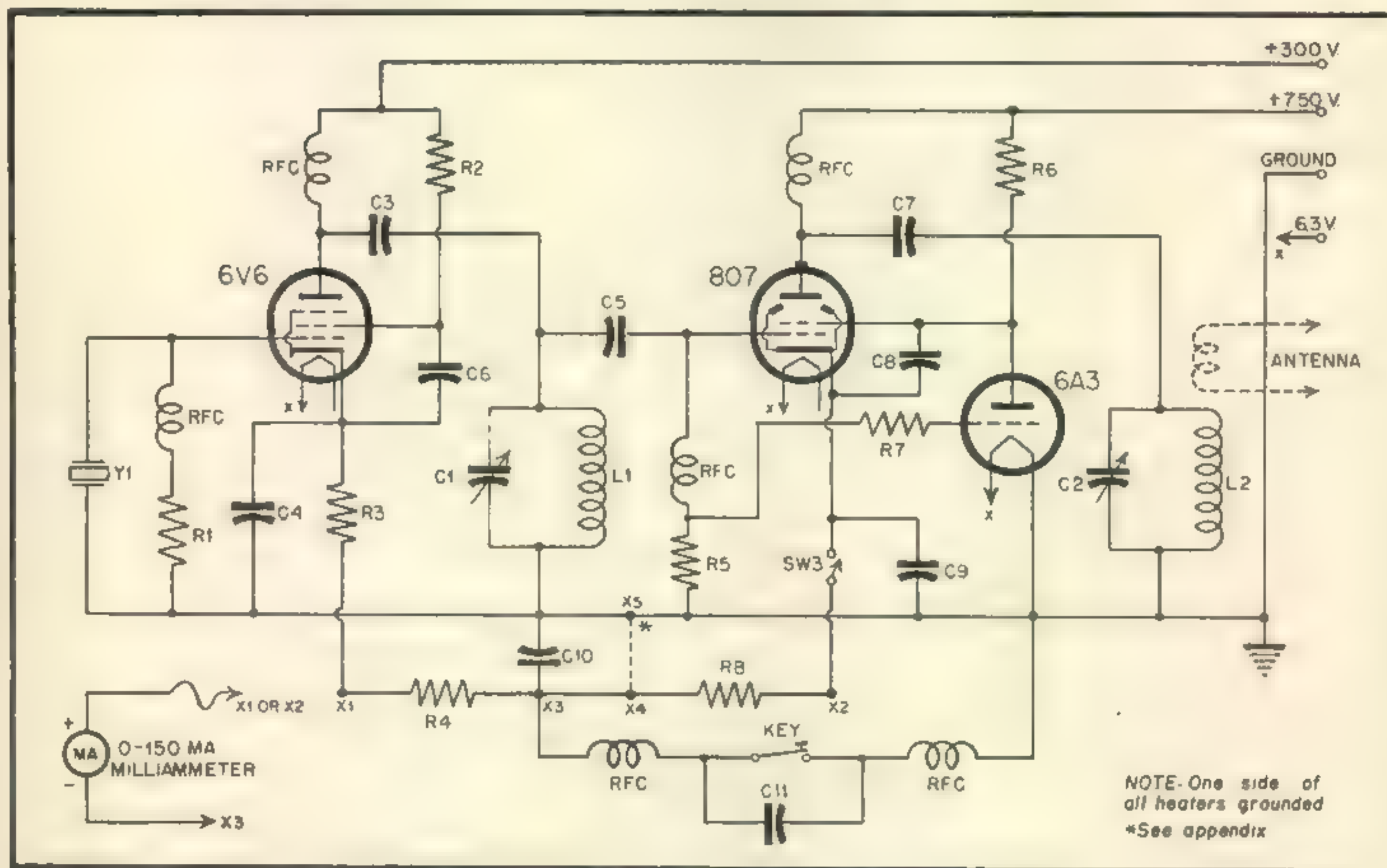
Fig. 1. Circuit diagram of the r-f end of the Watt Squeezzer I.
