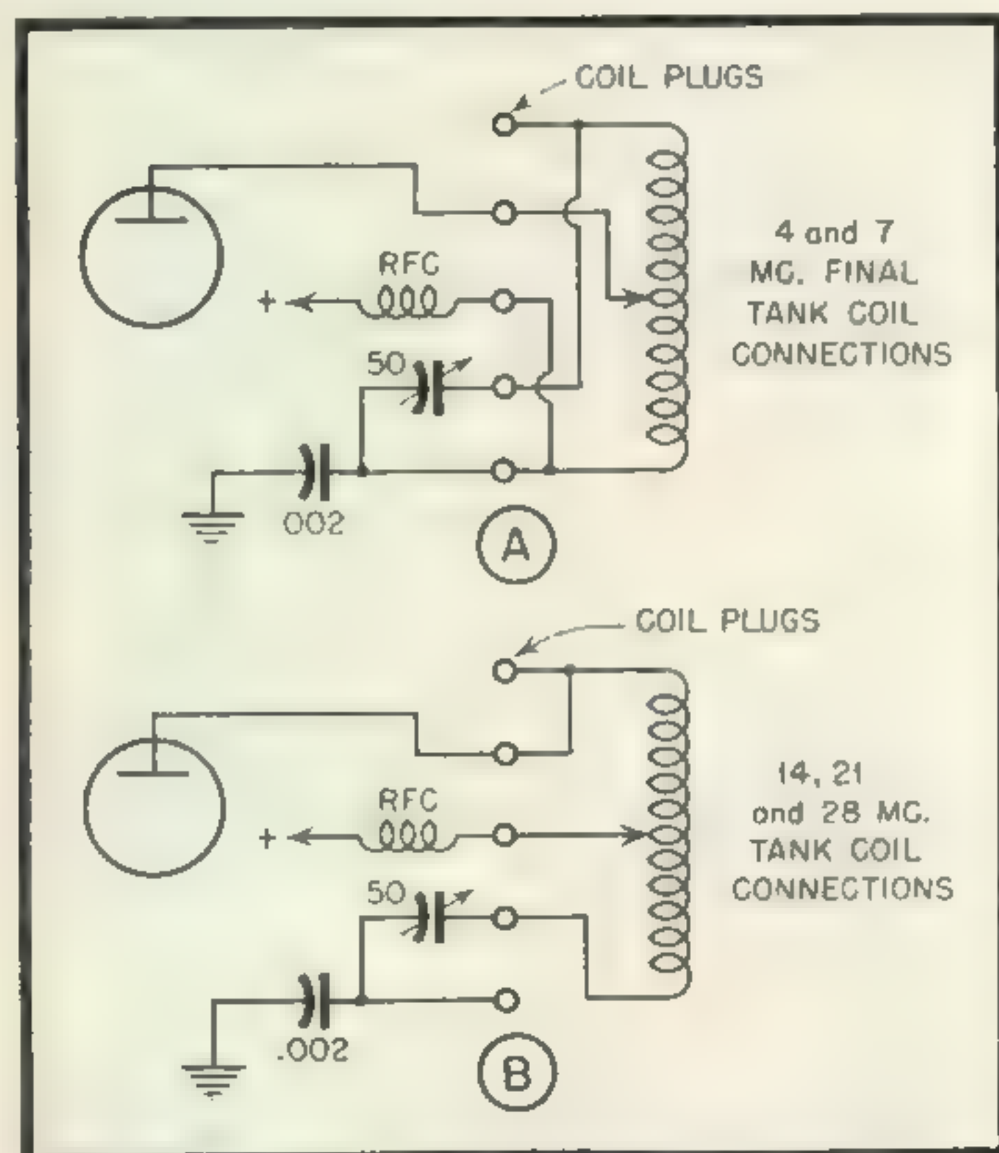
Fig. 3. Method of strapping connections between coil plugs on standard plug-in coils. Strapping as shown on top (A) gives parallel circuit drawn in Fig. 2 . Connected as shown on bottom (B) gives basic series tuned circuit of Fig. 1 .
