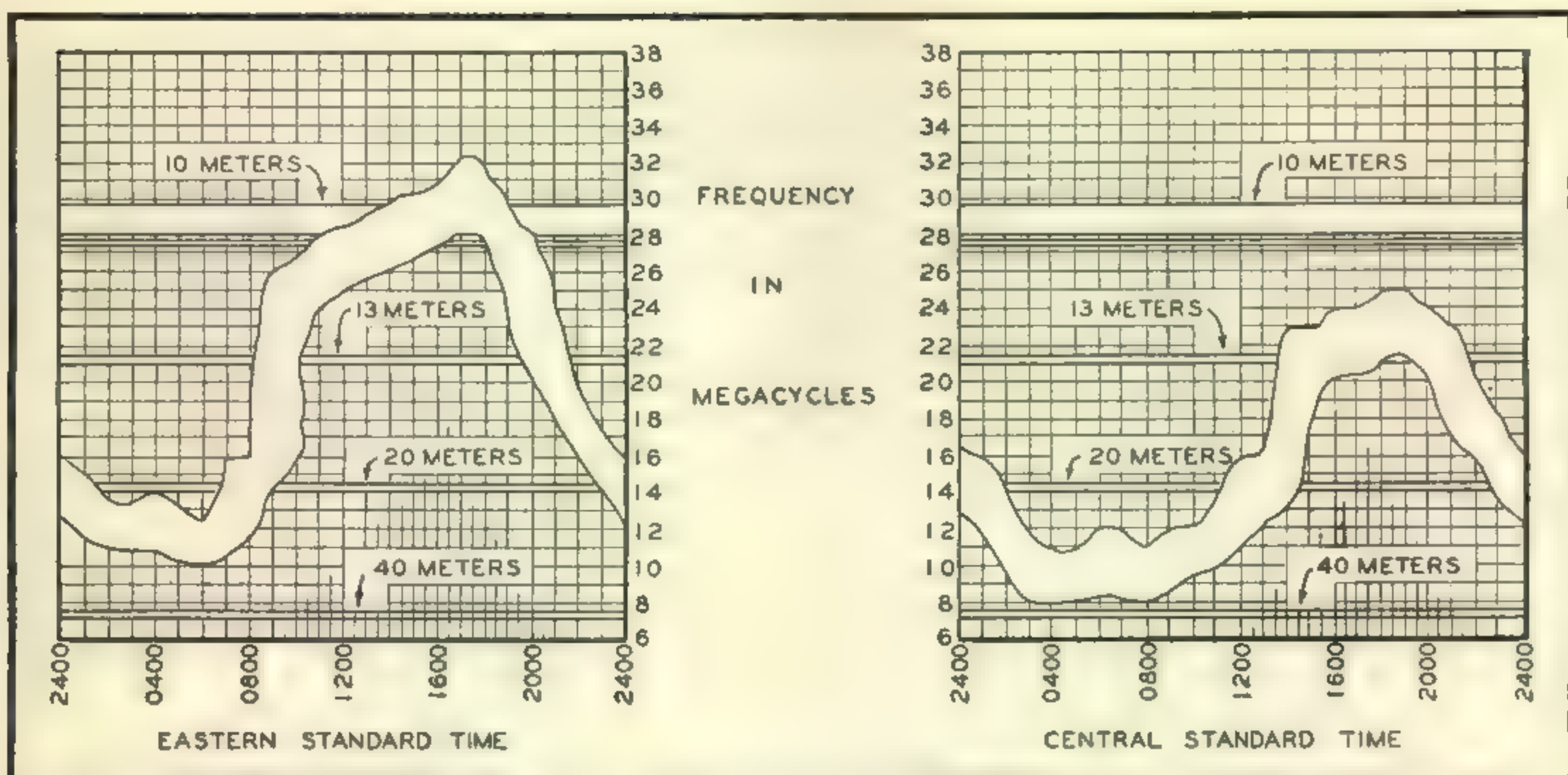
Fig. 2. (left) MUF and OMF East coast to West coast of United States, September 1946 average. Fig. 4. (right) MUF and OMF Central United States to Japan, September 1946 average.
