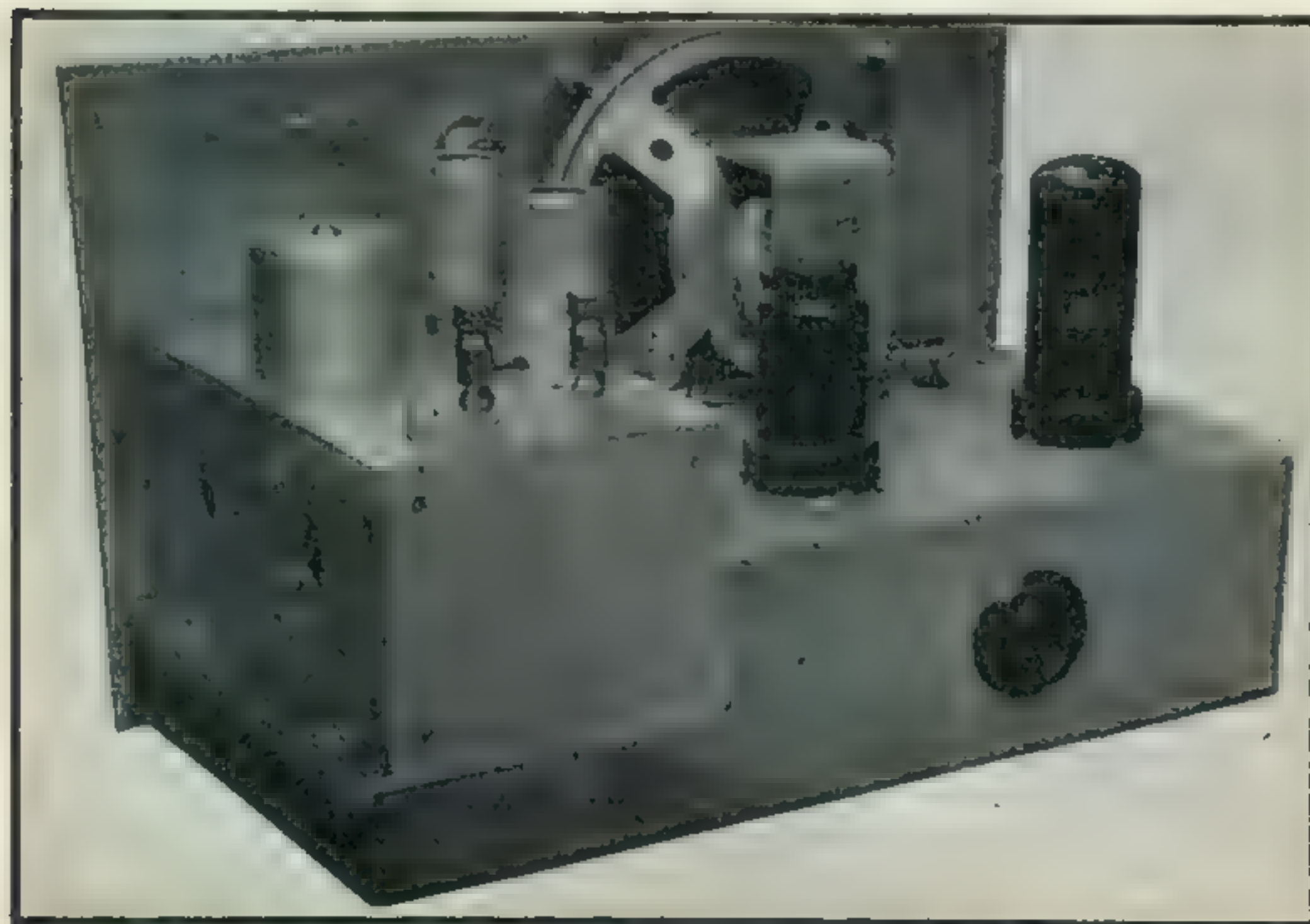
The entire r-f section is contained in a small aluminum box. Rigid mechanical connections will add stability. Components are located for minimum length leads .
