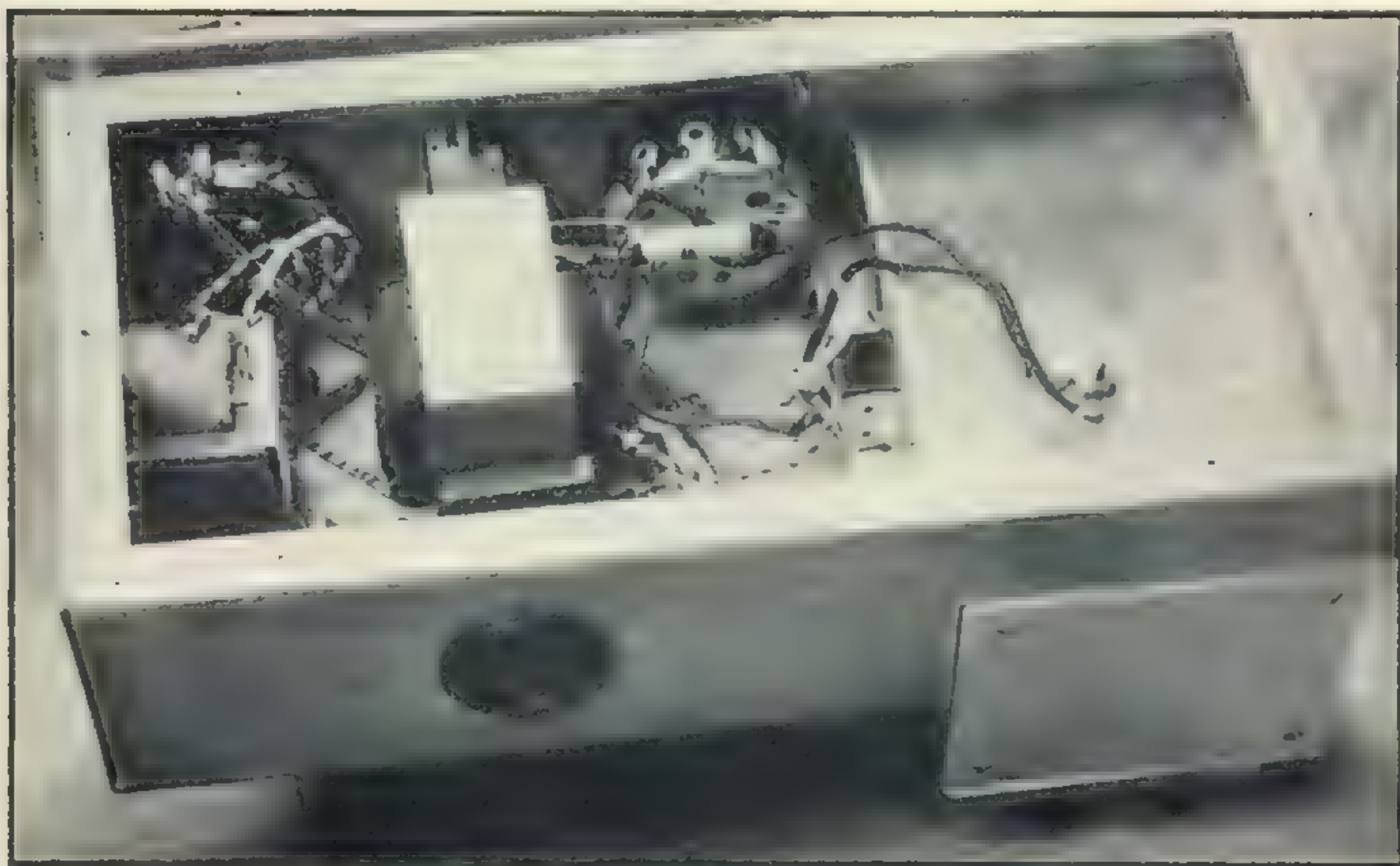
Underneath the audio-chassis. Placement of components is not critical because there is no r-f wiring in this section. The wires running to the side of the chassis containing the r-f section are common grounds and not extended through the chassis.
