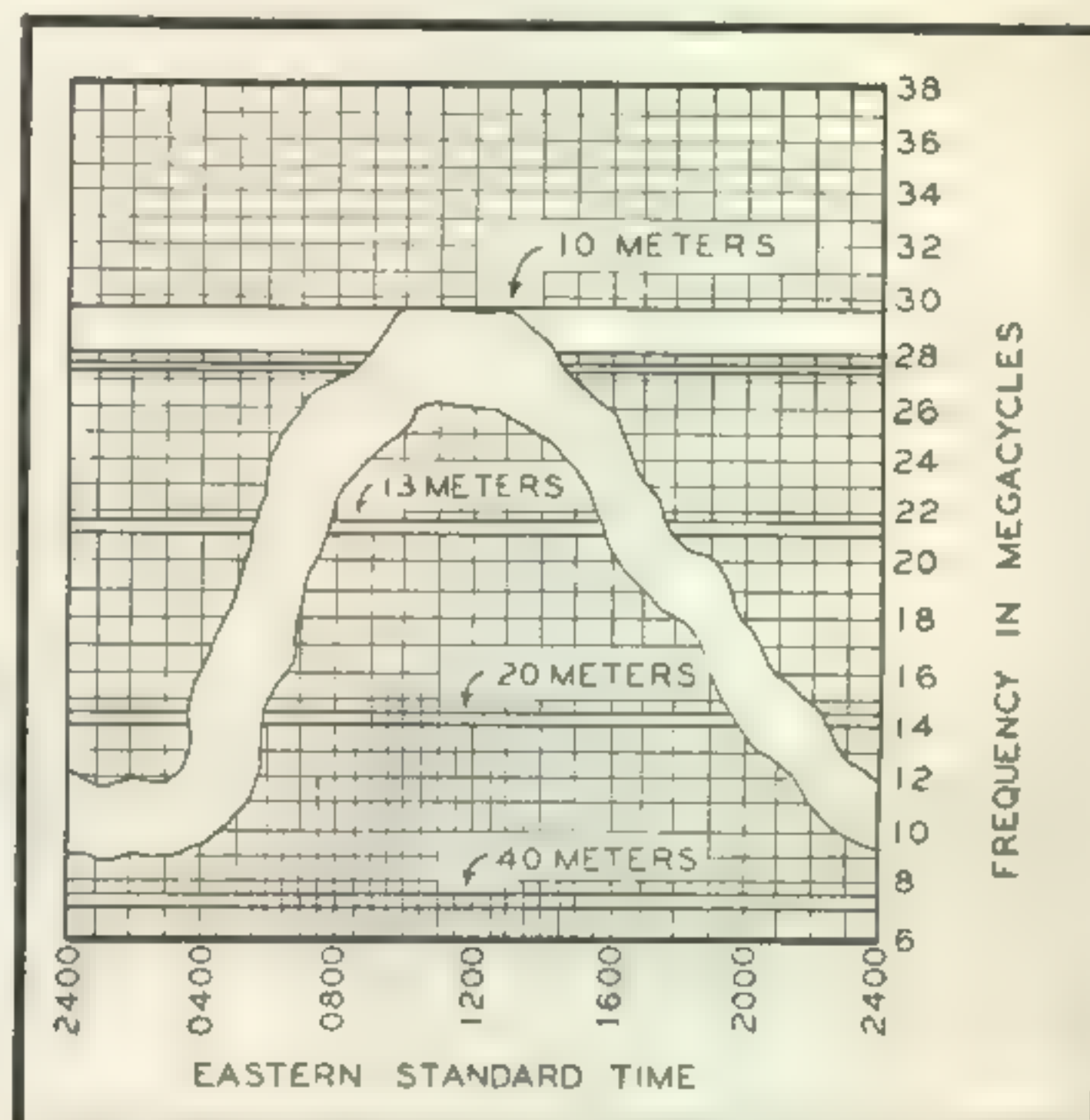
Fig. 3. MUF and OWF Eastern half of United States to Europe. September 1946 average
