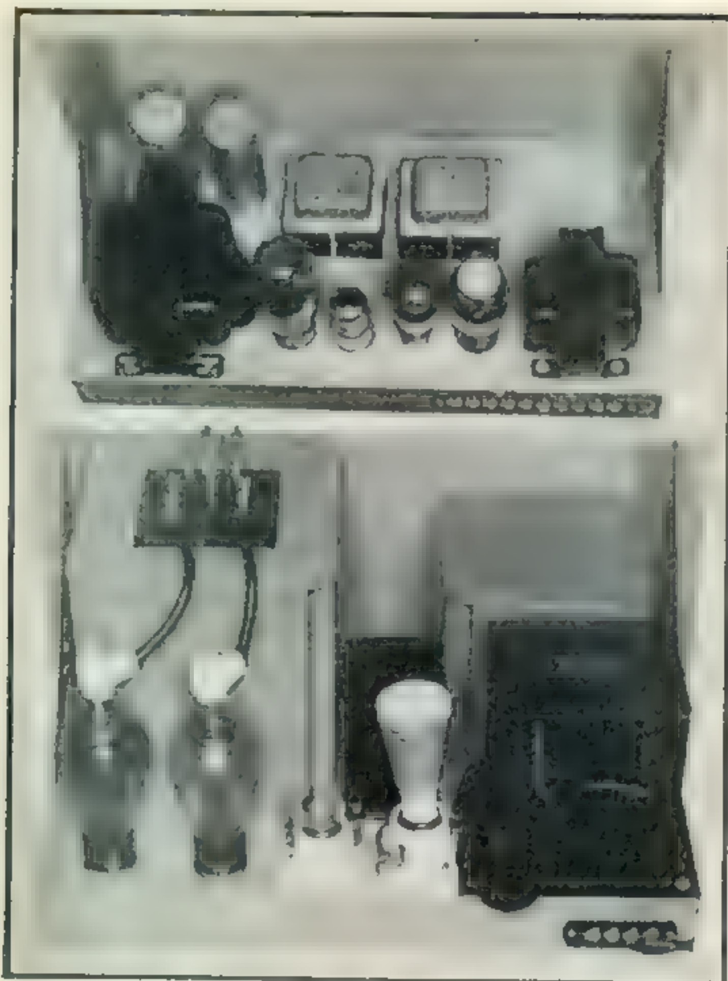
(Top) Low voltage power supply and bias supply. (Bottom) High voltage power supply for final amplifier and TZ-40 modulators. Heating unit may be switched in series with primary to lower plate voltage for tuning up transmitter or operating at reduced input.
