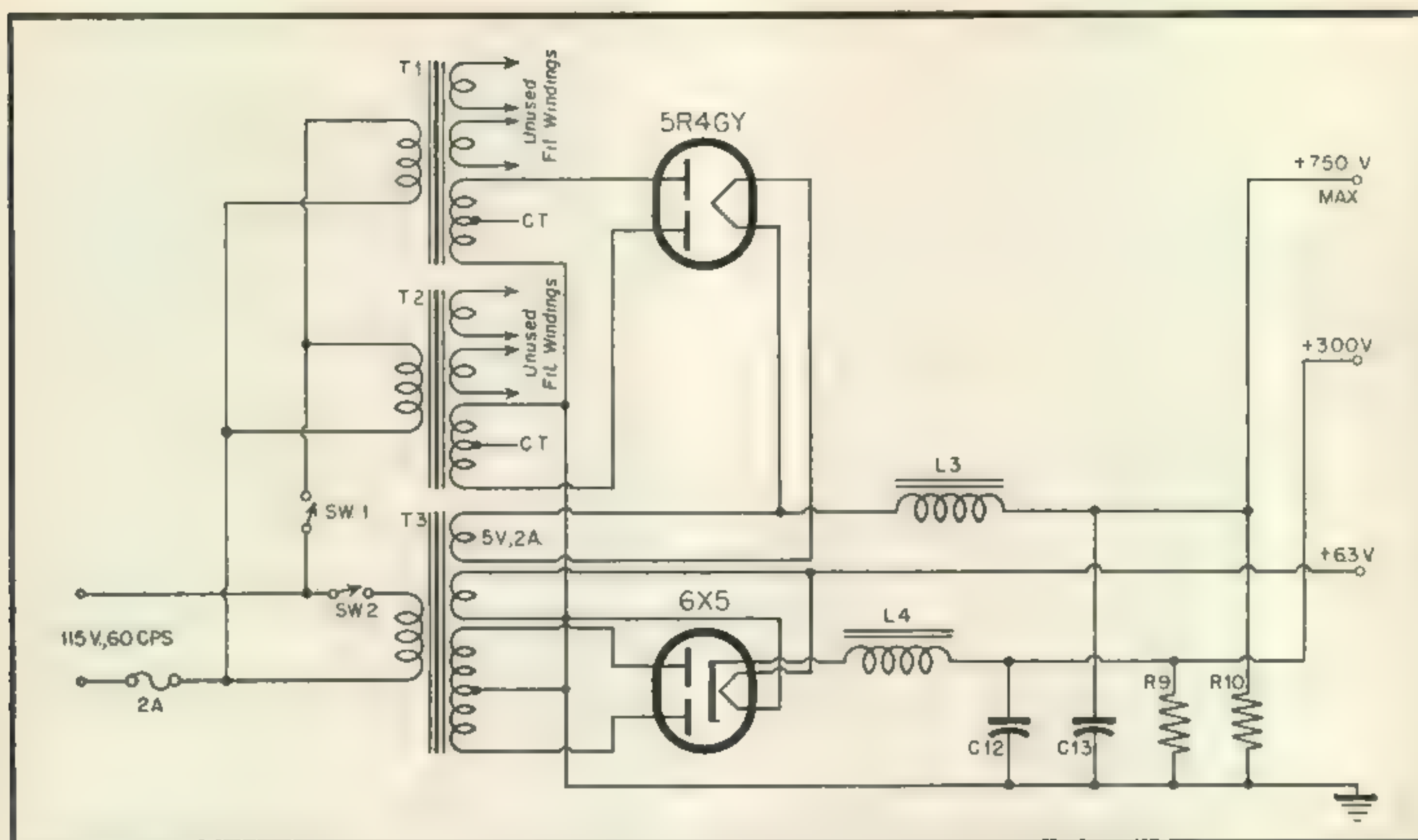
Fig. 2. Watt Squeezer I, Power Supply
