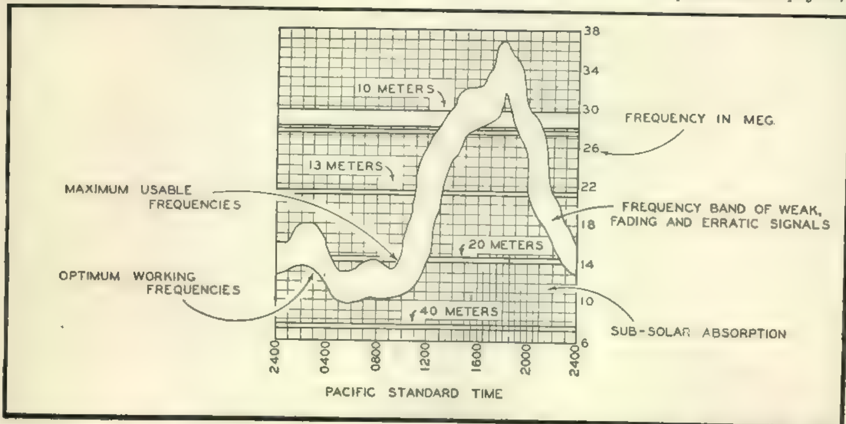
Fig. 1. Sample graph illustrating new method for presenting monthly DX predictions. Use of graphs is fully explained in text. This sample is based on the West Coast of United States to New Zealand and Australia. September 1946 average.
