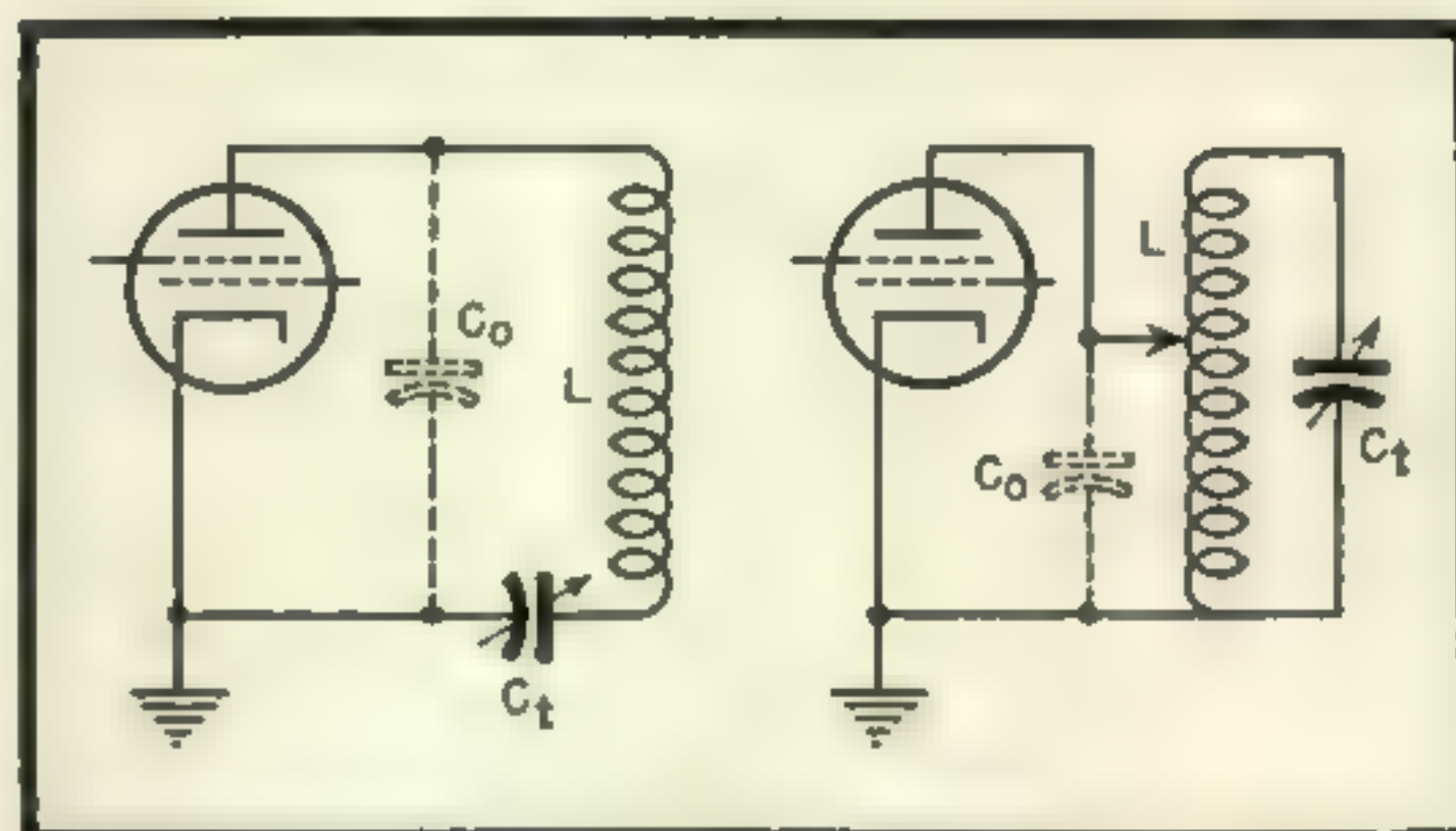
Fig. 1. (left) Basic series tuned circuit employed in final amplifier. Fig. 2 (right) Connections for parallel tuning accomplished by strap connections on coil plugs.
