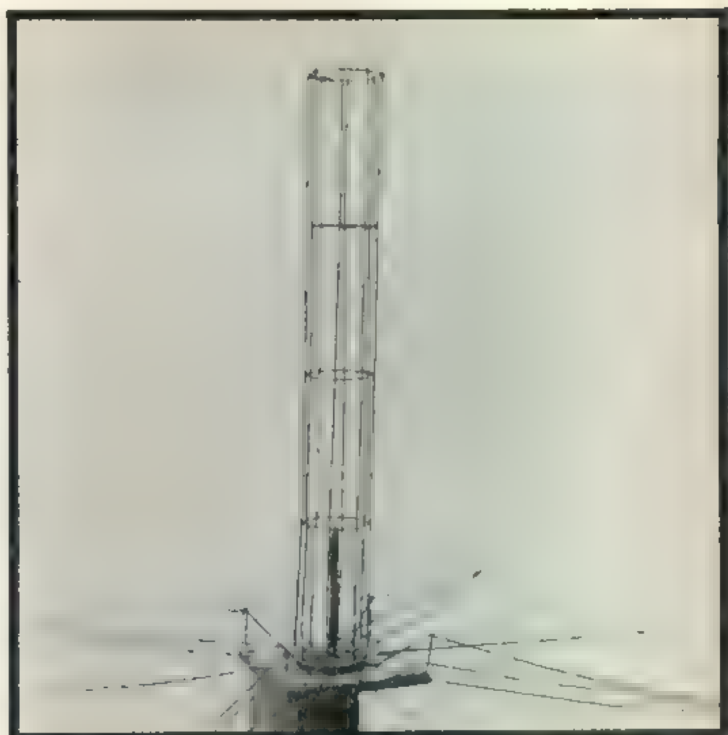
Broad-band two-meter ground-plane vertical antenna at W3GKP, Silver Spring, Md.
