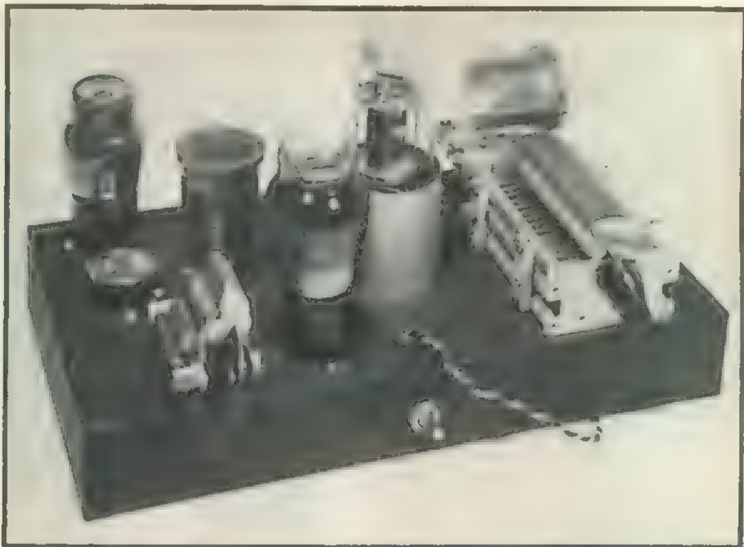
The Watt Squeezer I is a compact low power transmitter. Mechanically it is extremely simple and can be constructed with a minimum of tools. Twisted cable is metering lead, external to the rig.
