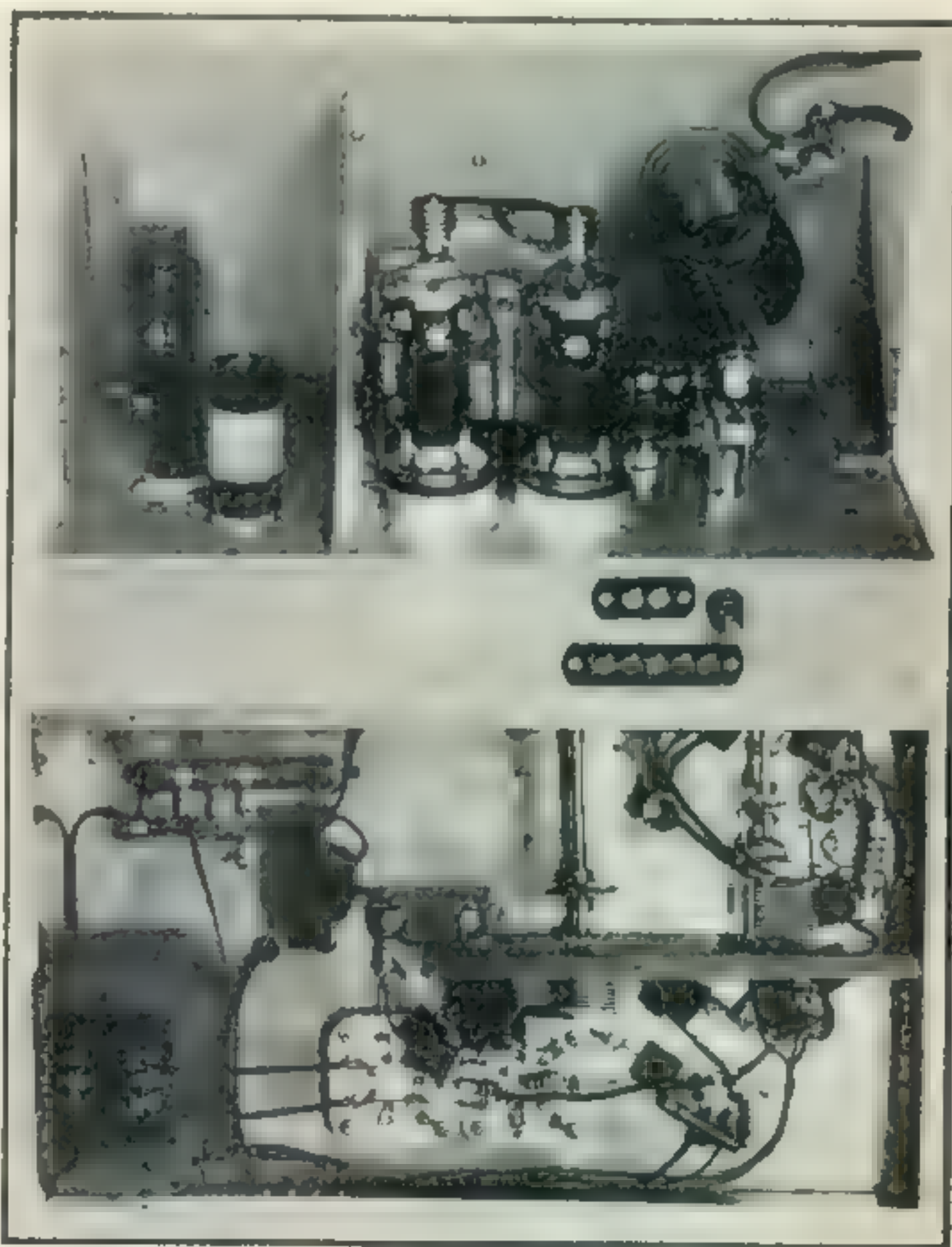
R-F unit is simple and straightforward in appearance. Parallel 813s are mounted side-by-side with common connections tied together.
